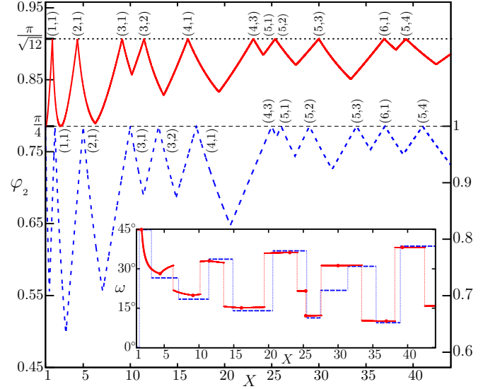
FIG. 2. (Color online). Maximum packing fraction \varphi_2(X) for rectangles (dashed line, right scale) and for ellipses (solid line, left scale). All global maxima lie on the dotted and dashed lines, respectively. Inset: orientation angle \omega as a function of X for rectangles (dashed line) and ellipses (solid line). The dots correspond to the position of the maxima of \varphi_2(X) for ellipses.
