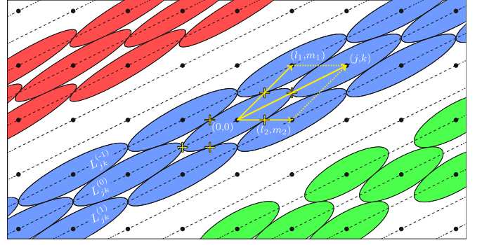
FIG. 3. (Color online). Maximum packing configurations of ellipses with aspect ratios X = 3 (green, bottom), X_{21}^{\max} = \sqrt{29 + 8\sqrt{13}}/\sqrt{3} \approx 4.39 (blue, middle), and X = 6 (red, top). Lattice lines for (j, k) = (2, 1) (dashed lines) and contact points (crosses).
