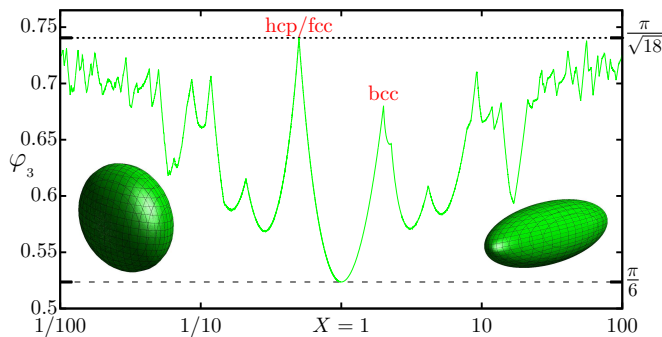
FIG. 4. (Color online). Maximum packing fraction for biaxial ellipsoids on an sc lattice on a logarithmic X scale. The dashed and dotted lines represent global minimal and maximal packing fractions, respectively.
