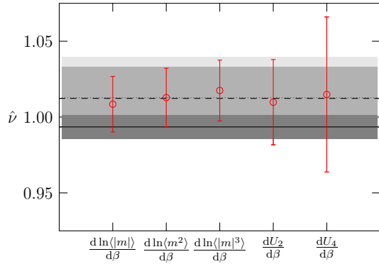
FIG. 1: (Color online) Estimates of the critical exponent \nu of the 2D Ising model from the FSS of the indicated observables. The horizontal lines indicate the plain average \bar{\nu}_{\text{plain}} (dotted), the error-weighted mean \bar{\nu}_{\text{err}} (dashed), and the covariance-weighted mean \bar{\nu}_{\text{cov}} (solid). The shaded areas indicate the corresponding one-sigma environments \bar{\nu} \pm \sigma_{\text{corr}} .
