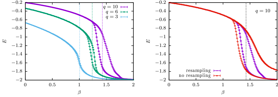
Figure 2. Left: Internal energy as measured in cooling runs (right curve of each color) and heating runs (left curve of each color) for q = 3 , q = 6 and q = 10 from PA runs for L = 32 and R = 10000 with \theta = 10 and \Delta\beta = 0.01 . It is clearly visible that hysteresis occurs in the first-order cases q = 6 and q = 10 , but not for the second-order model with q = 3 . The vertical dashed lines show the asymptotic transition points at \beta_t = \ln(1 + \sqrt{q}) . Right: The data for q = 10 as shown on the left compared to the data for equivalent PA runs with the resampling step turned off.
