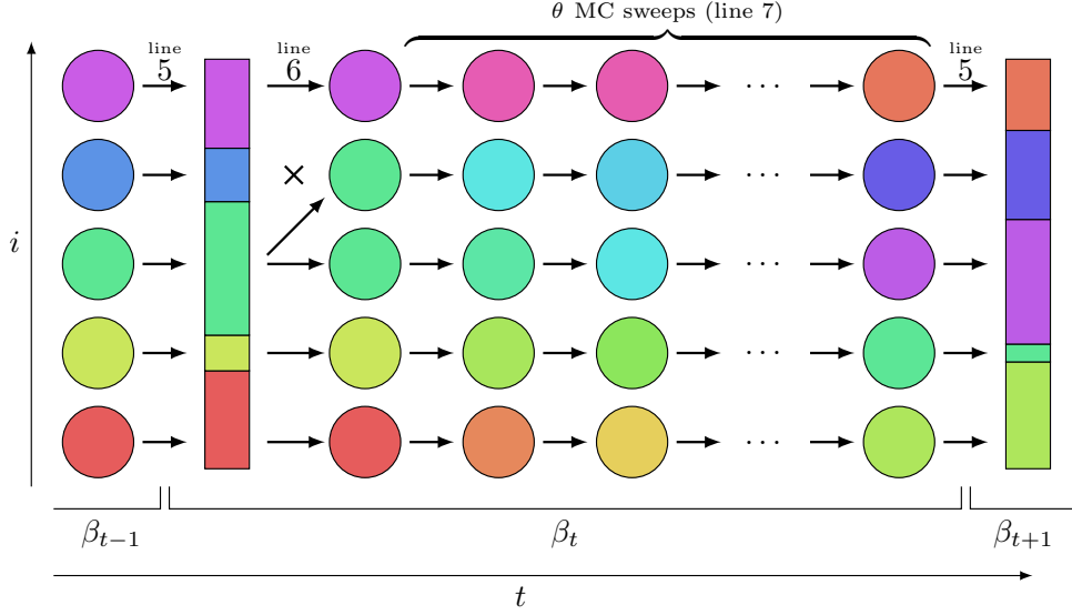
Figure 1. Schematic of the population annealing algorithm. Vertical axis corresponds to R replicas (here five) and horizontal axis to simulation time. Line numbers correspond to algorithm 1 in Appendix A.
