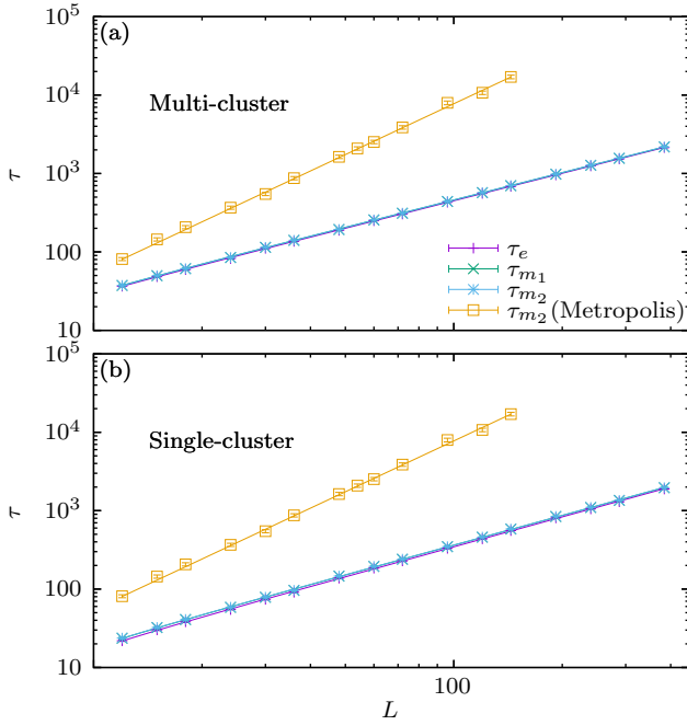
FIG. 7. Scaling behavior of the integrated autocorrelation times for the energy and the two order parameters defined in Eqs. (8) and (9). The dynamical critical exponent z is extracted via fits to the scaling form in Eq. (17). Panel (a) shows results for the multi-cluster update, while panel (b) corresponds to the single-cluster update. For comparison, Metropolis results for m_2 are also included. All curves exhibit an overall linear trend, with the single-cluster data displaying a slightly steeper slope than the multi-cluster results.
