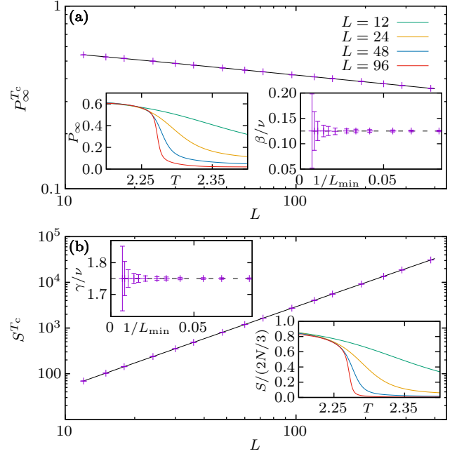
FIG. 6. FSS of (a) the percolation strength P_\infty and (b) the average cluster size S , including the largest cluster. Both observables are evaluated at the Ising-model critical temperature (11). Power-law fits yield the critical exponent ratios \beta/\nu and \gamma/\nu , respectively. The insets show the estimated exponents as a function of L_{\min} , with horizontal dashed lines indicating the exact values \beta/\nu = 1/8 and \gamma/\nu = 7/4 . Also included are insets with the corresponding curves of P_\infty and the normalized cluster size S/(2N/3) .
