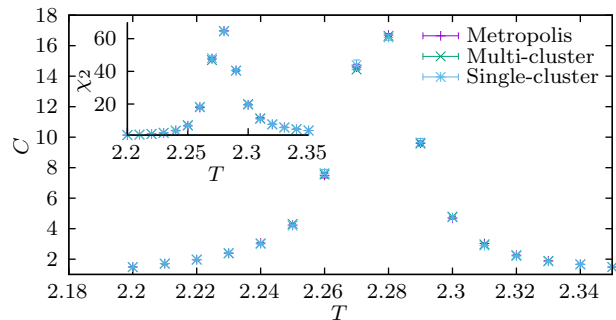
FIG. 3. Comparison of simulation results obtained using the Metropolis, single-cluster, and multi-cluster updates for the specific heat and magnetic susceptibility of the spin-1/2 BW model at various temperatures for a system of linear size L = 48 . The main panel shows the specific heat C(T) , while the inset displays the magnetic susceptibility \chi_2(T) . The excellent agreement between the methods confirms the correctness of the cluster-algorithm implementation.
