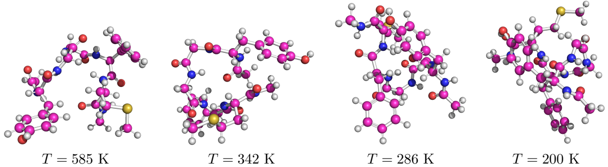
Figure 1. Snapshots of Met-enkephalin at different temperatures, decreasing from left to right. The following color-code applies: pink – carbon, white – hydrogen, red – oxygen, blue – nitrogen, yellow – sulfur.
