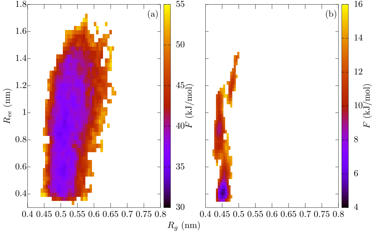
Figure 3. Plots of the end-to-end distance versus the radius-of-gyration for our simulation of Met-enkephalin at (a) T = 700 K and (b) T = 200 K.
