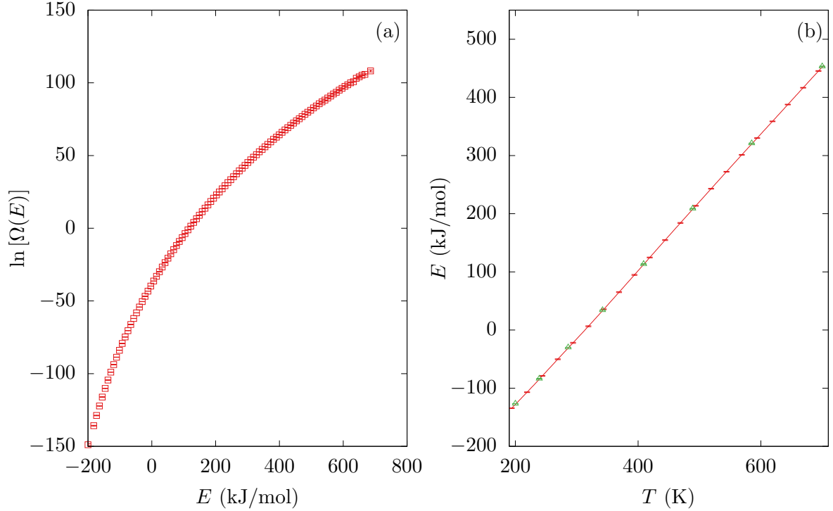
Figure 2. (a) Logarithm of the density of states for Met-enkephalin obtained from our PAMD simulation using WHAM [33, 34, 35]. (b) (Potential) energy E as derived from the density of states of (a) as a function of temperature T . The green triangles indicate population averages at the actual simulation temperatures.
