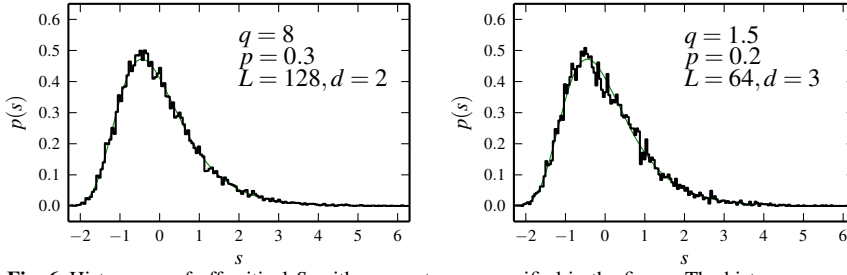
Fig. 6 Histograms of off-critical S , with parameters as specified in the figure. The histograms are based on 19,000 independent samples for d = 2 and 11,000 for d = 3 . Here p(s) denotes the probability density function of S . For comparison, the solid green line shows the probability density function corresponding to (2.19).
