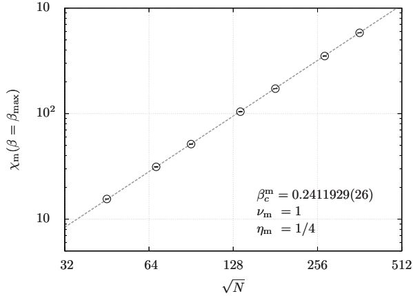
FIG. 1: Log-log plot of the FM susceptibility at its peaks, \chi_m(\beta = \beta_{\max}) , as a function of the effective linear system size \sqrt{N} . The data fall onto a straight line, showing that corrections to scaling are very small. The dashed line has slope 2 - \eta = 7/4 .
